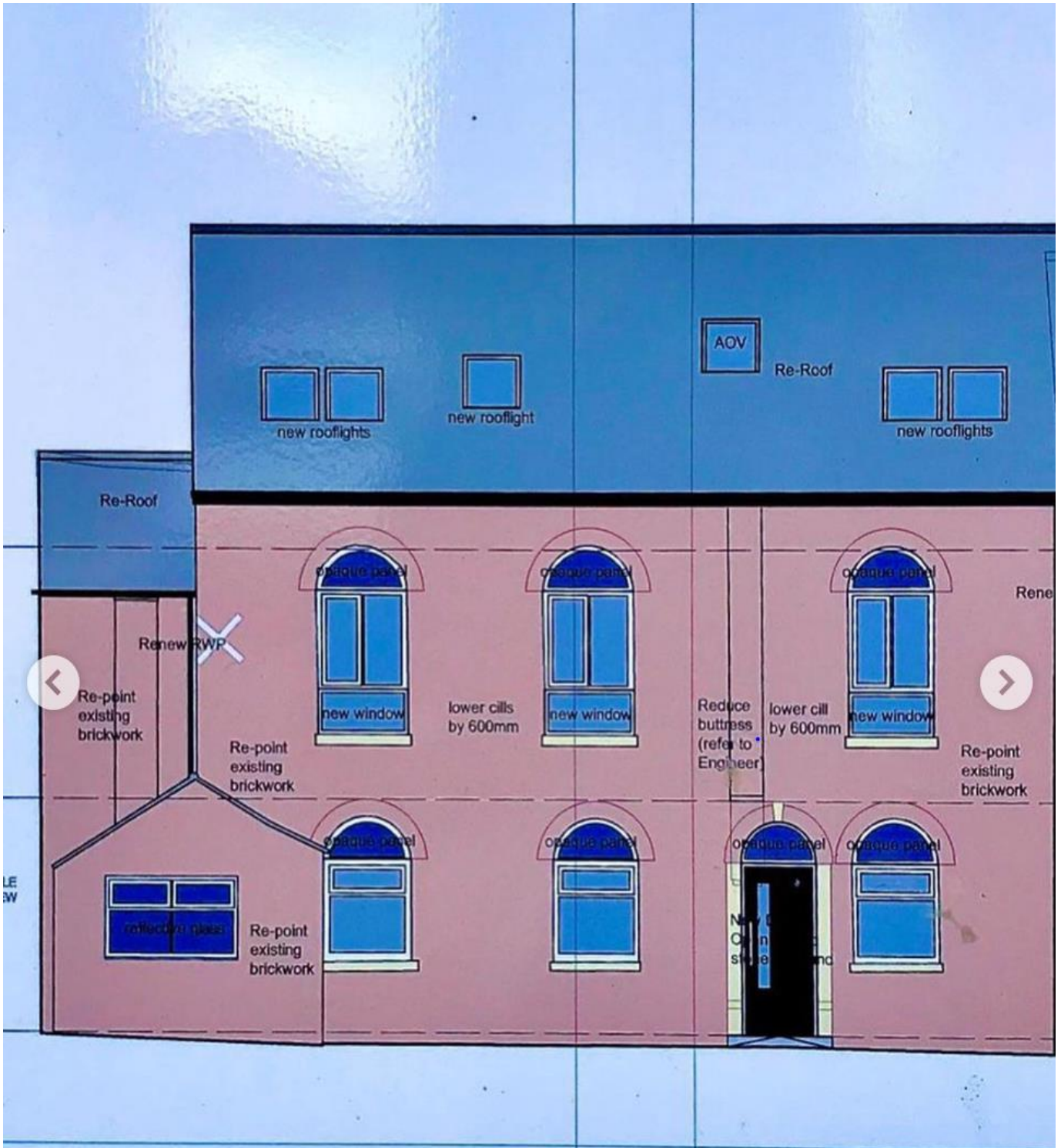
Elevation to Sunningdale Road
